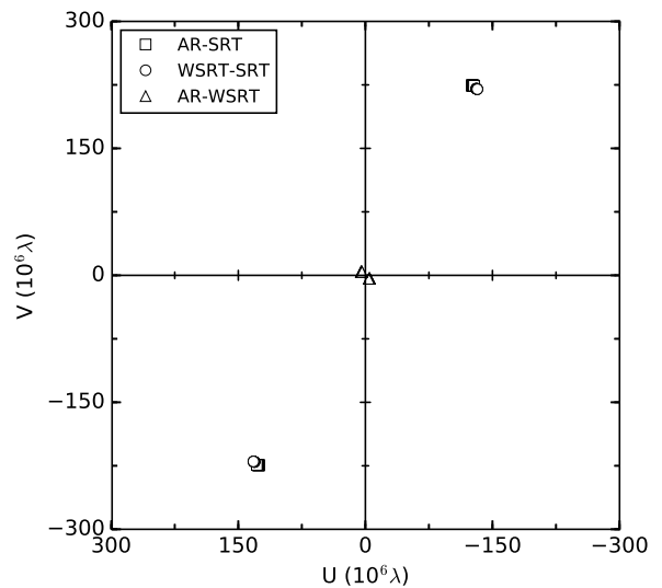
Figure 2. UV-coverage (visibility coverage of the Fourier domain) obtained for RadioAstron observations of PSR B0950+08 in units of spatial frequency, defined as the projected baseline in wavelengths 10^6\lambda .
