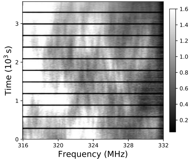
Figure 1. Dynamic cross-spectrum of PSR B0950+08 at an observing frequency of 324 MHz for the Arecibo-WSRT ground baseline
