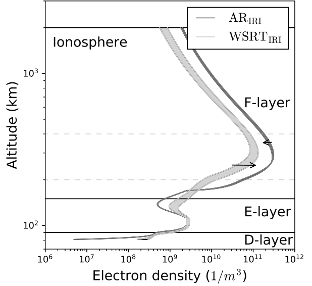
Figure 5. Profiles of ionospheric electron density from IRI at 05-06 UT on 25 th January, 2012 at the positions of the Arecibo and WSRT stations. The arrows indicate the directions along which the profile changes. The ionospheric layers are shown. The ionospheric profile extends up to a height of 2,000 km.
